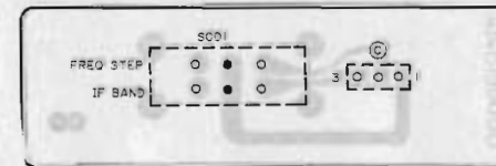
IFS/DU Switch P.C.B. Ass'y (OTR)
