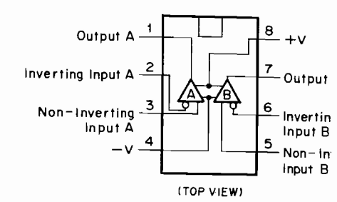
Fig. 7.1.5 Operational Amp. NJM2043DD, \mu P
