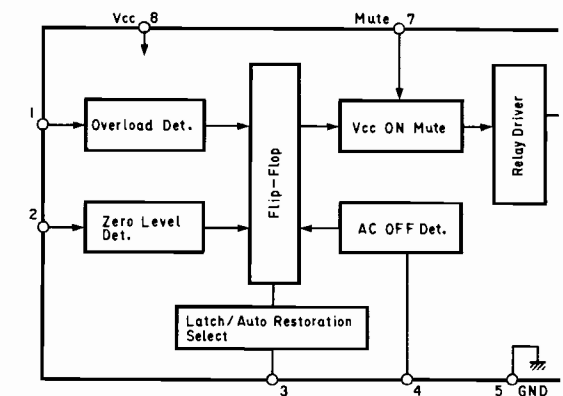
Fig. 7.1.7 Power Amp. Protector \mu PC1237 (U301)
