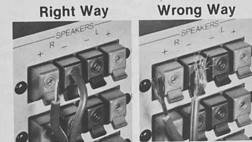
Wire Stripping: Strip off only ¼-inch of insulation. Stripping more than that will leave bare wire exposed and could cause a damaging short circuit.
