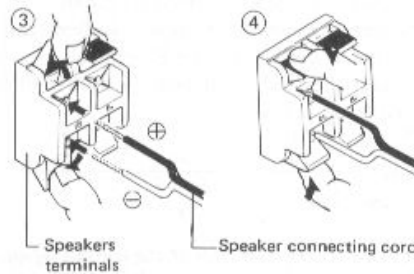
Fig.6 - SPEC-1 FROM POWER AMP and SPEAKERS terminals.
