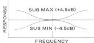
Fig.14 - SUB Tone control characteristic.
