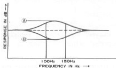
Adding slight body to low frequencies
