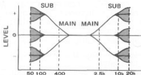
Adjusting first the main, then the sub controls can provide the range of adjustment shown by the shaded areas in the figure.
