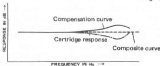
Compensation for cartridge high frequency "hollowness"
