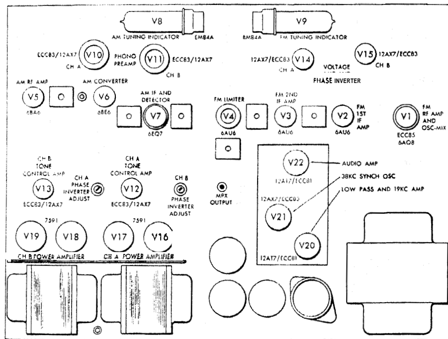
FIGURE 2. Tube layout.
