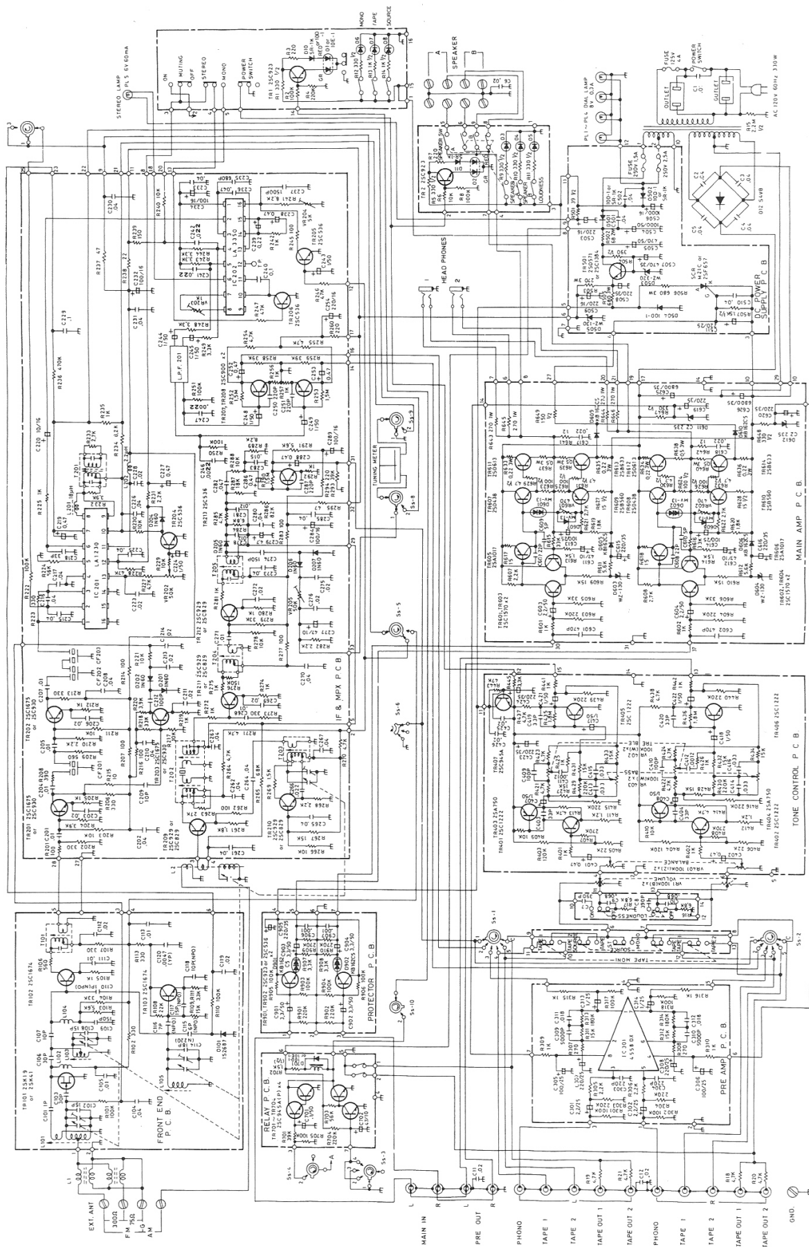
SCHEMATIC DIAGRAM
