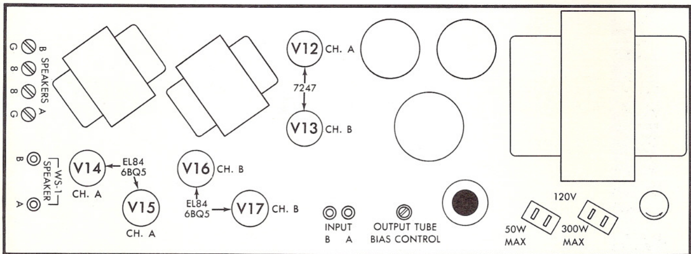
AMPLIFIER
